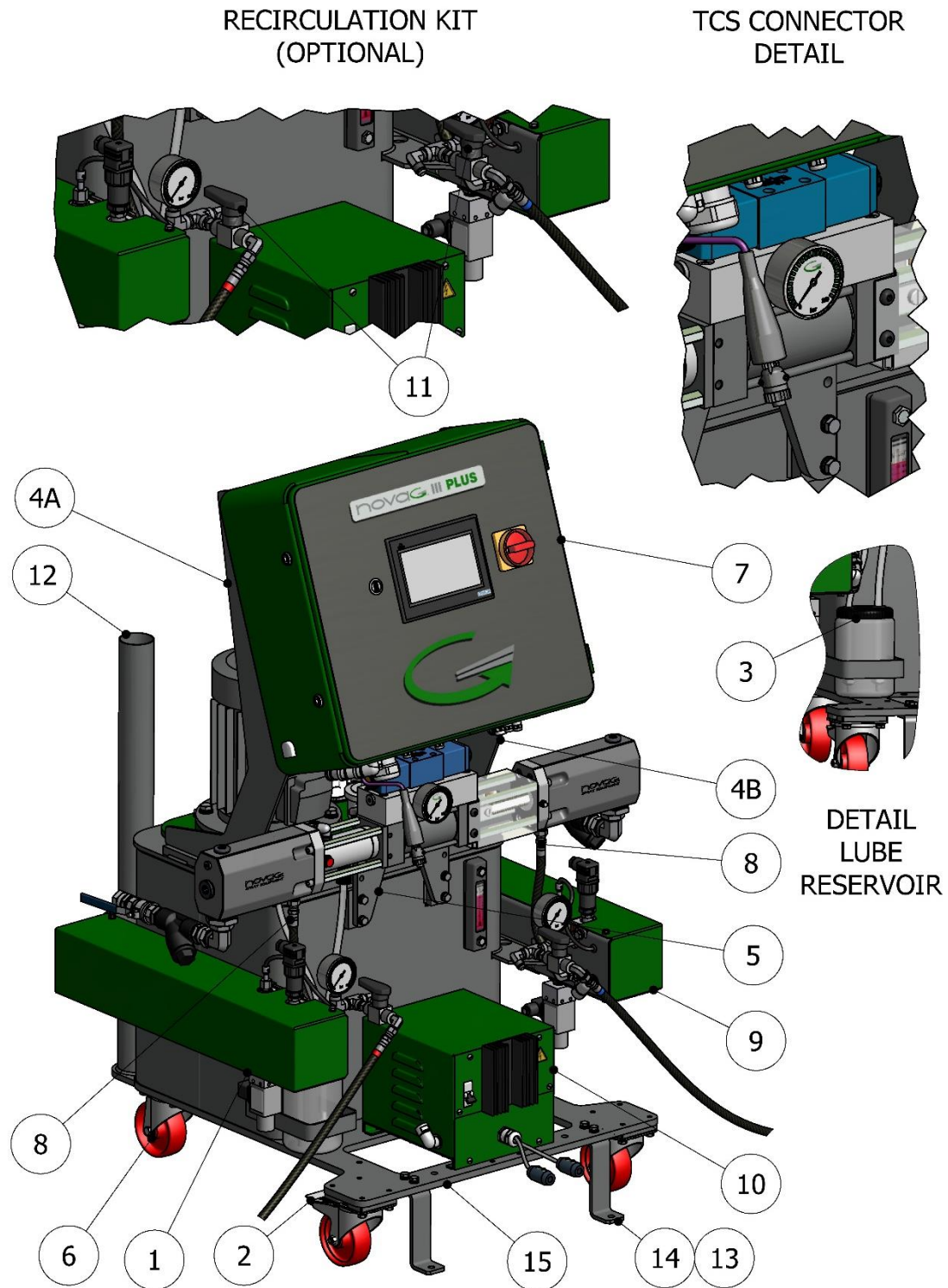
Figure 1. Proportioning Unit novaG III PLUS Model
