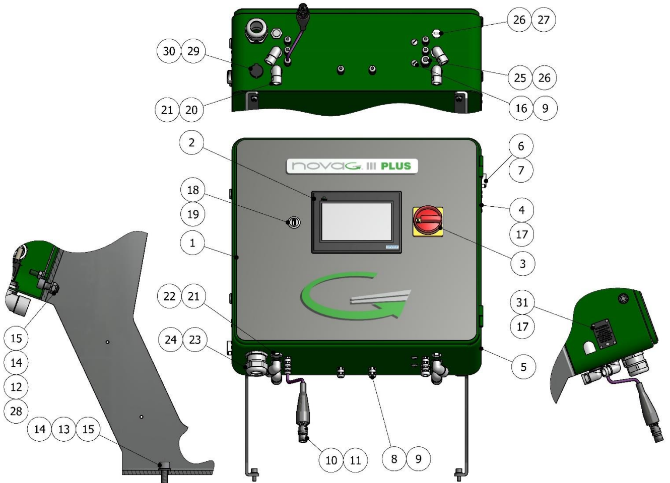
Figure 1. Electrical Console novaG III PLUS
